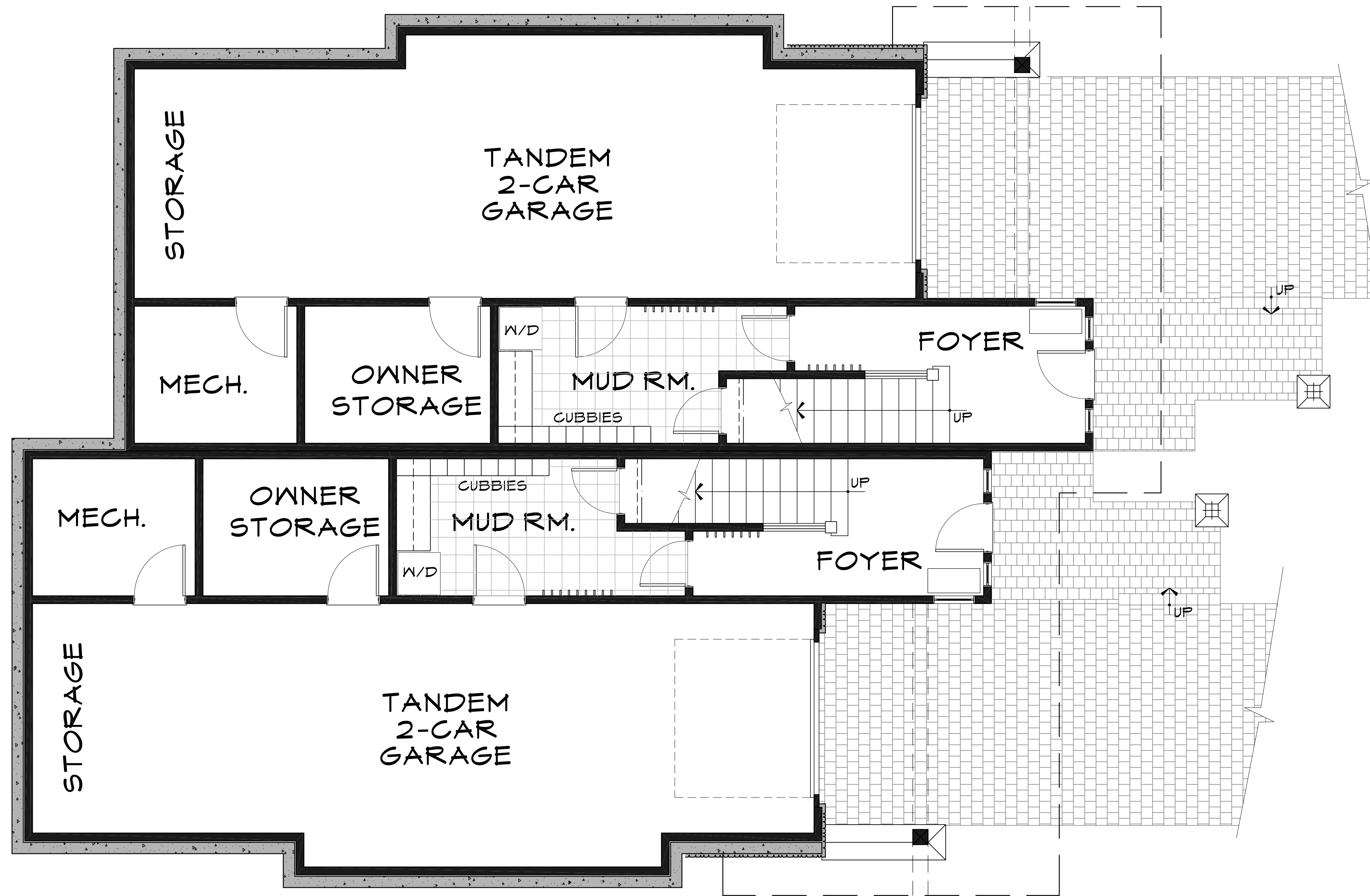
LOWER LEVEL FLOOR PLAN
