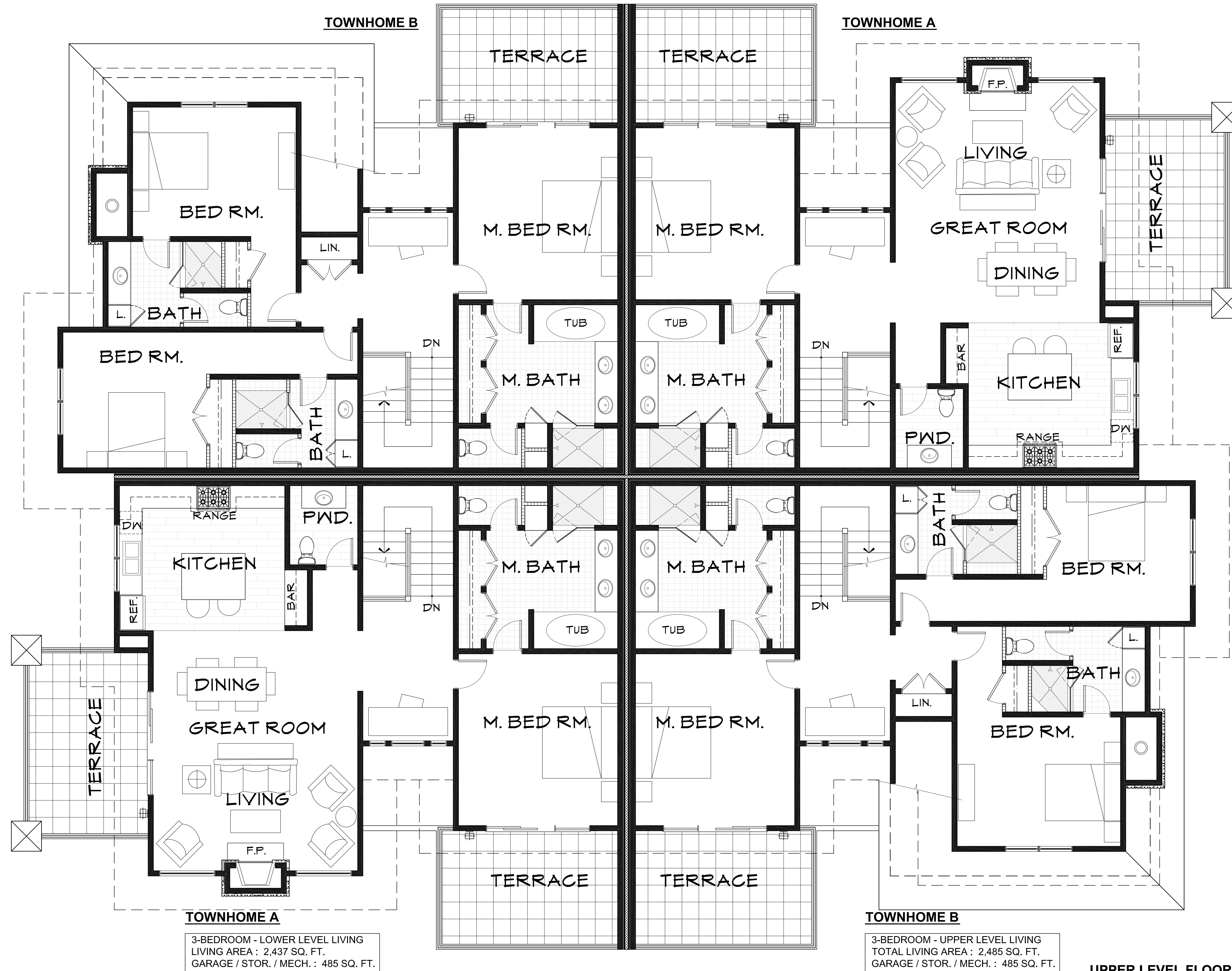
UPPER LEVEL FLOOR PLAN
